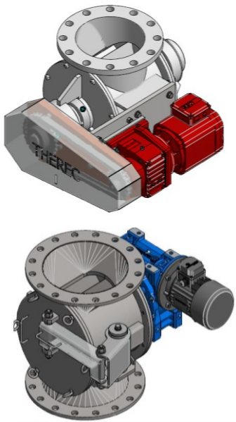
Air Lock Rotary Valve
